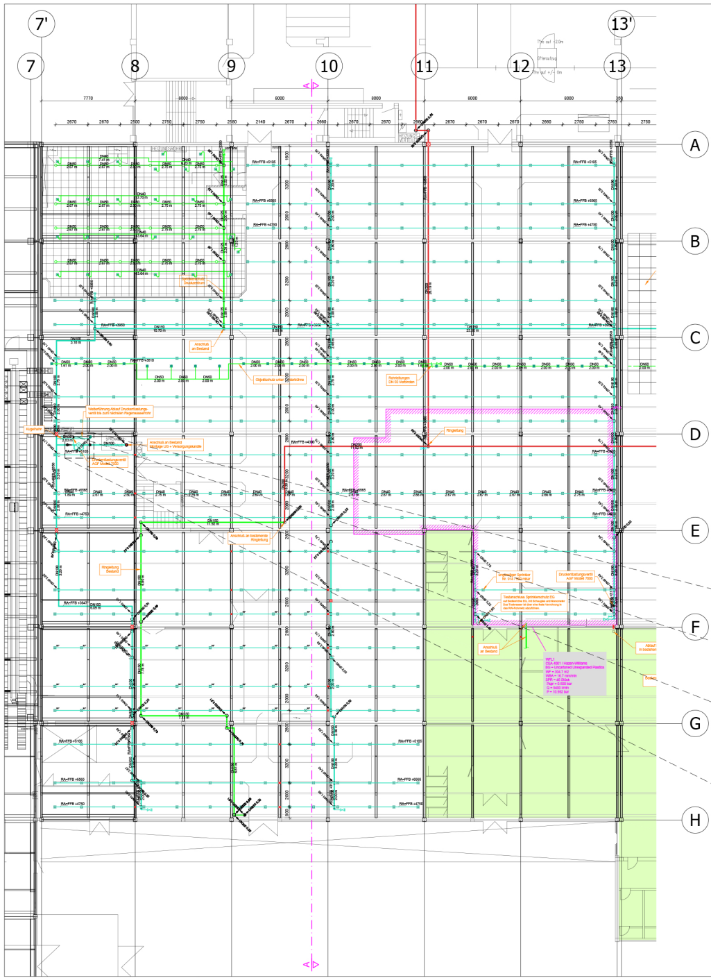
Grundriss M 1:100 0 1.0 2.0 3.0
